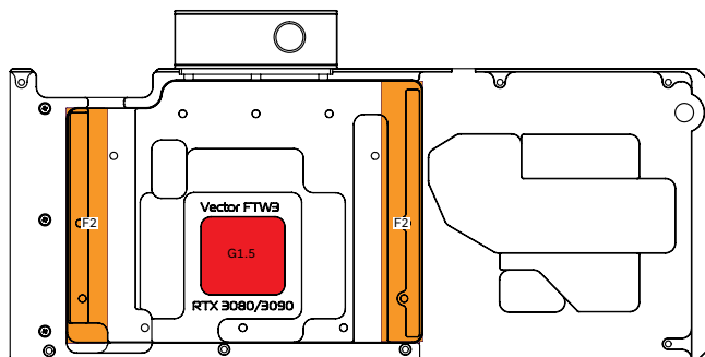
G1.5 Thermal Pad G 1.5 mm
