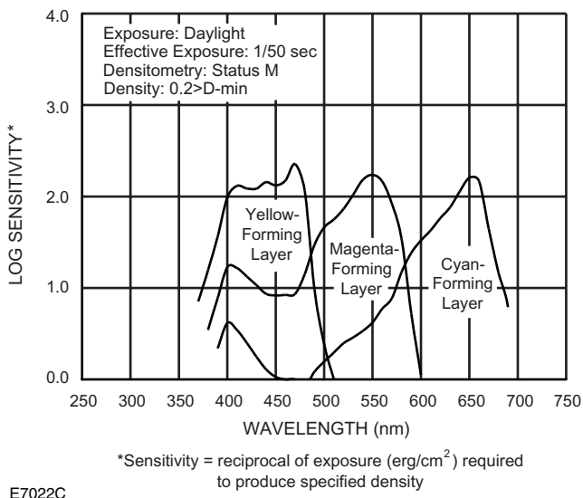
Spectral-Sensitivity Curves
