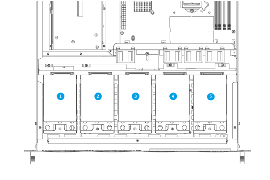
2.5-inch Drive Bays
