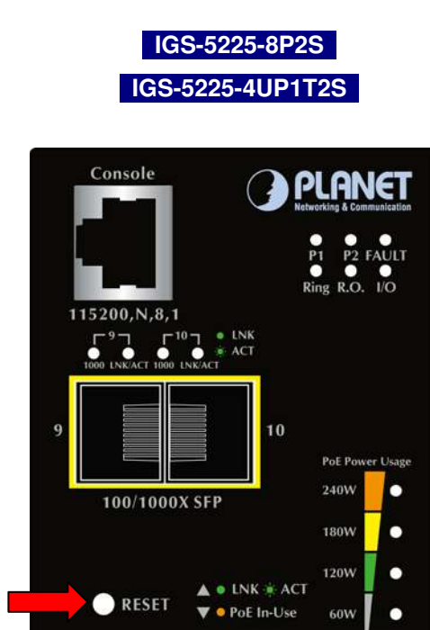
Figure 2-8: IGS-5225-8P2S/IGS-5225-4UP1T2S Reset Button
