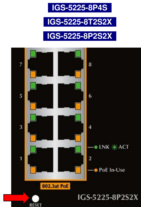
Figure 2-9: IGS-5225-8P4S/IGS-5225-8T2S2X/ IGS-5225-8P2S2X Reset Button
