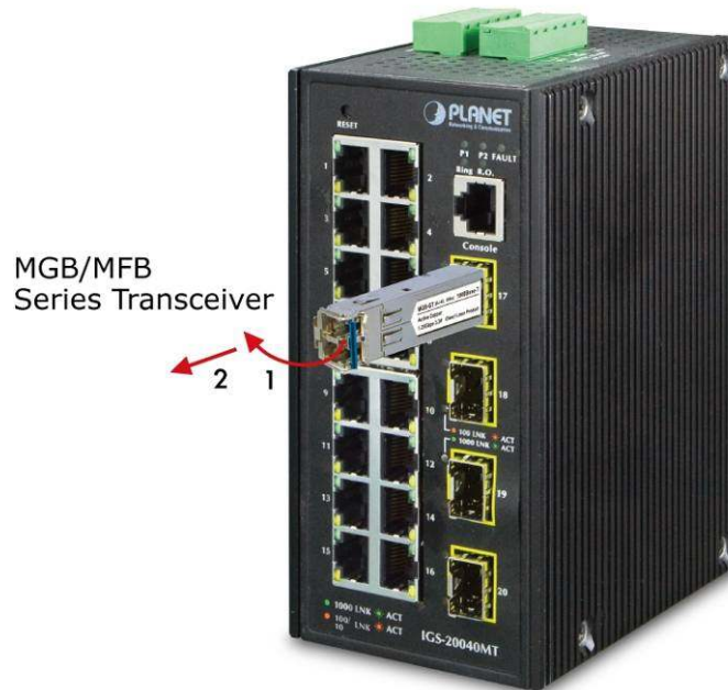
Figure 2-26: Pull out the SFP/SFP+ Transceiver Module
