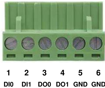
Figure 2-15 6-pin Terminal Block for DI and DO Wiring Input
