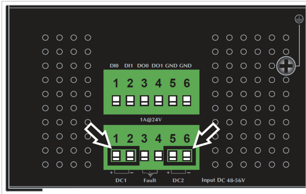
Figure 2-10: IGS-5225-8P2S/IGS-5225-8P4S/IGS-5225-8P2S2X/IGS-5225-4UP1T2S Upper Panel
