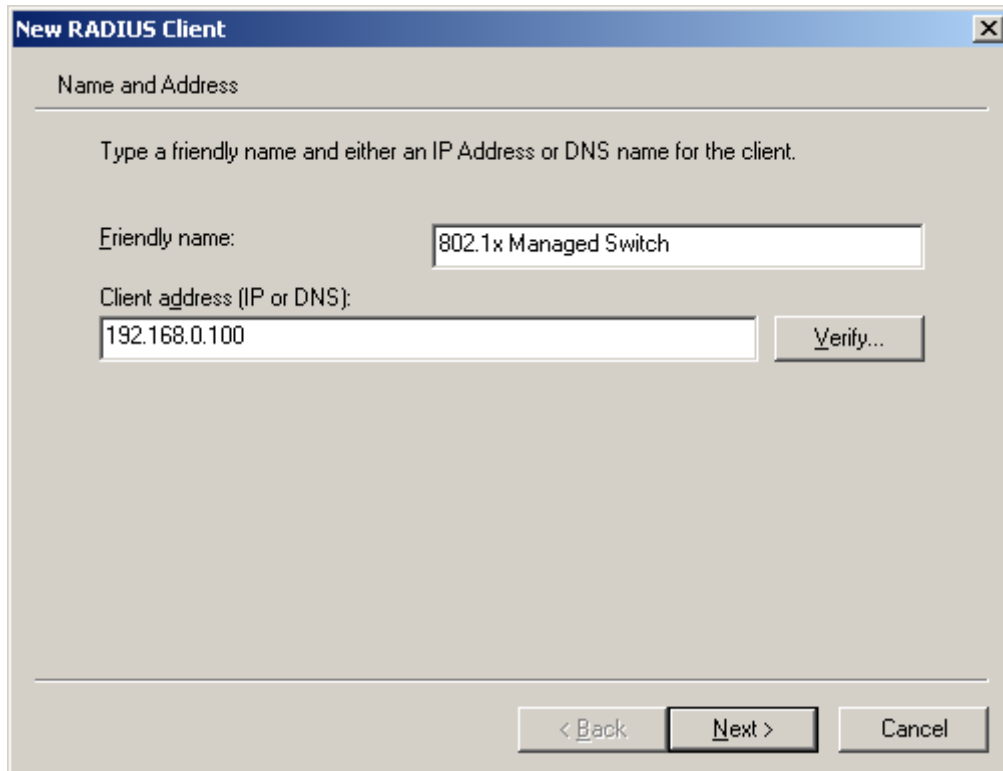
Figure 4-11-16: Windows Server RADIUS Server Setting
