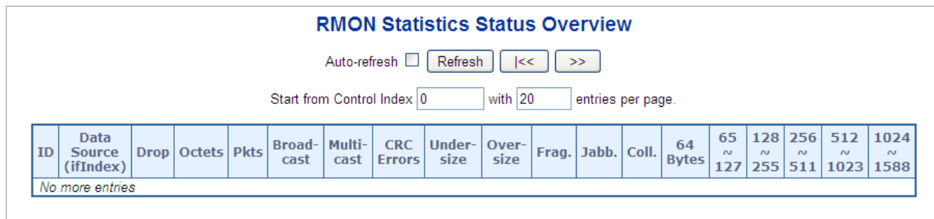
Figure 4-18-8: RMON Statistics Status Overview page Screenshot
