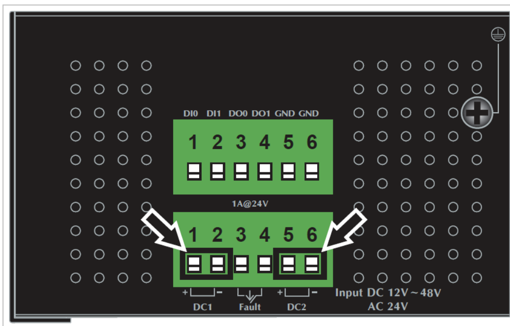
Figure 2-11: IGS-5225-8T2S2X Upper Panel
