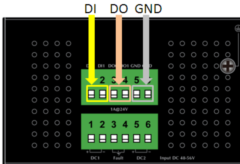
Figure 2-14 Wiring the Redundant Power Inputs
