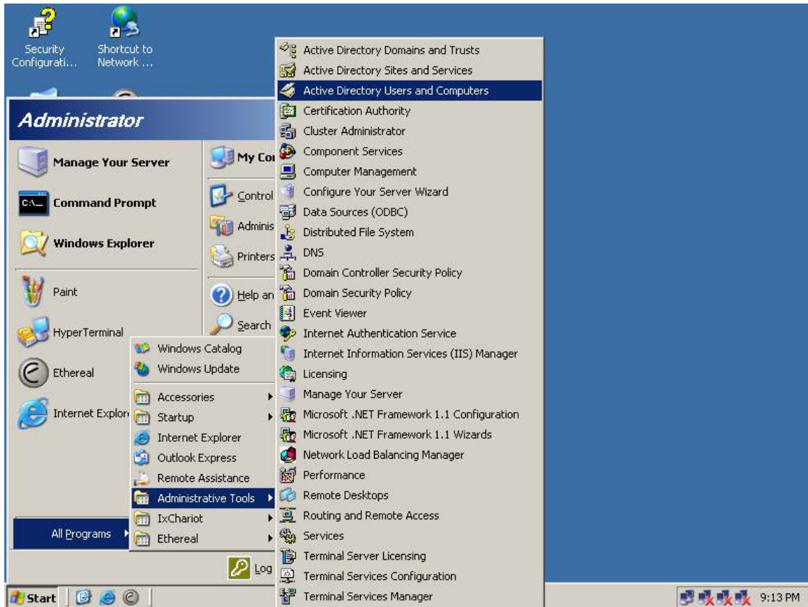
Figure 4-11-19: Windows 2003 AD Server Setting Path
