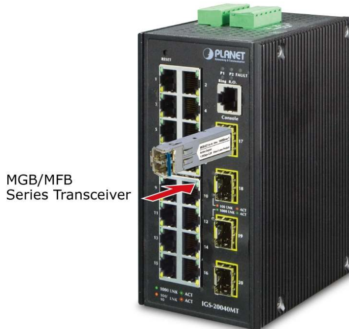
Figure 2-18: Plug in the SFP/SFP+ Transceiver
