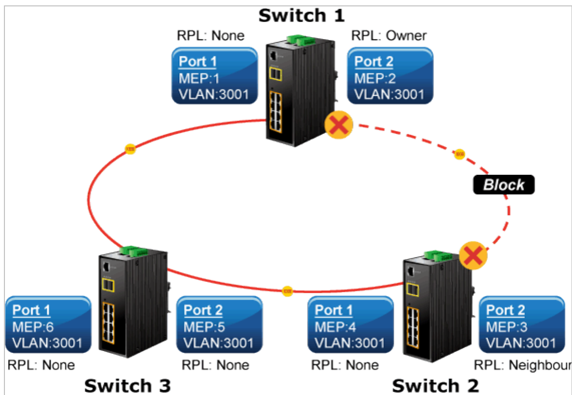
Figure 4-20-6: Ring Example Diagram
