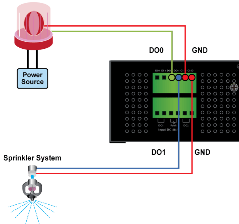
Figure 2-17 Wires DO0 and DO1 to Open Detector
