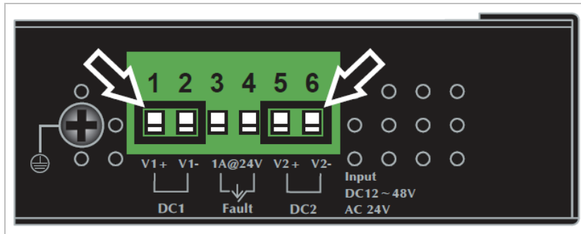
Figure 2-12: IGS-5225-4T2S Upper Panel
