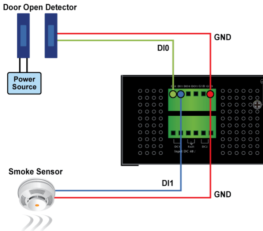
Figure 2-16 Wires DI0 and DI1 to Open Detector
