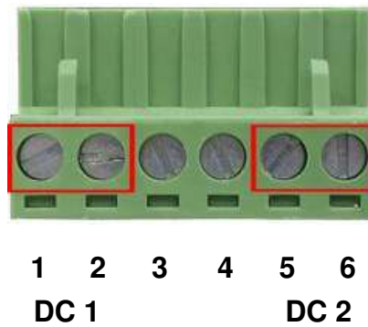
Figure 2-13 6-Pin Terminal Block Power Wiring Input
