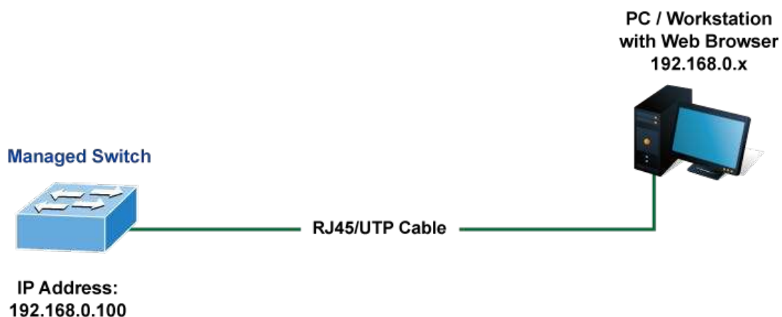
Figure 4-1-1: Web Management
