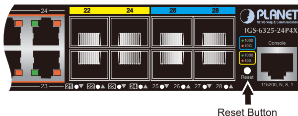
Figure 6-3: IGS-6325-24P4X and IGS-6325-24P4S Reset Button
