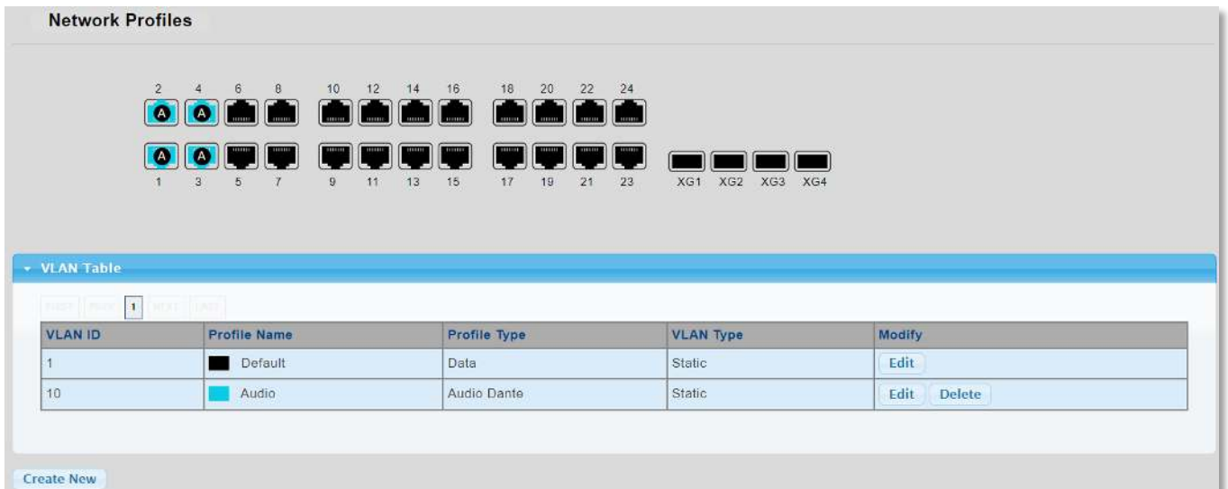
Figure 4-5-25: Complete audio VLAN configuration
