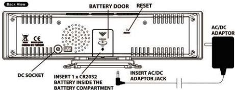
Back View
