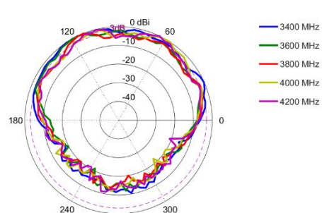
Elevation: 3400 – 4200 MHz
