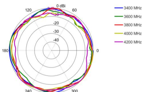
Azimuth: 3400 – 4200 MHz
