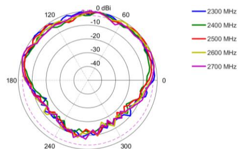
Elevation: 2300 – 2700 MHz
