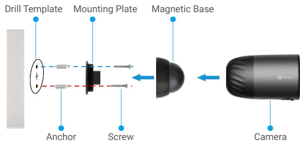
Fig. 2 Secure by magnetic base
