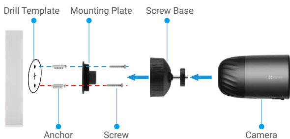
Fig. 1 Secure by screw base
