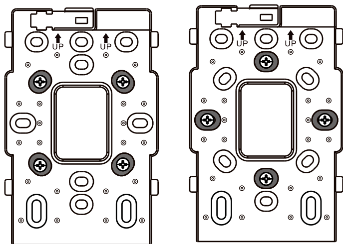
Bracket on European-standard 86 mm × 86 mm Junction Box
