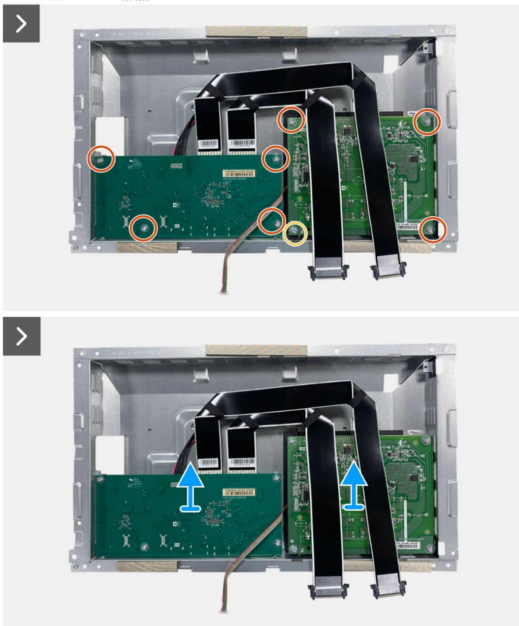
Figure 37. Removing the interface board
