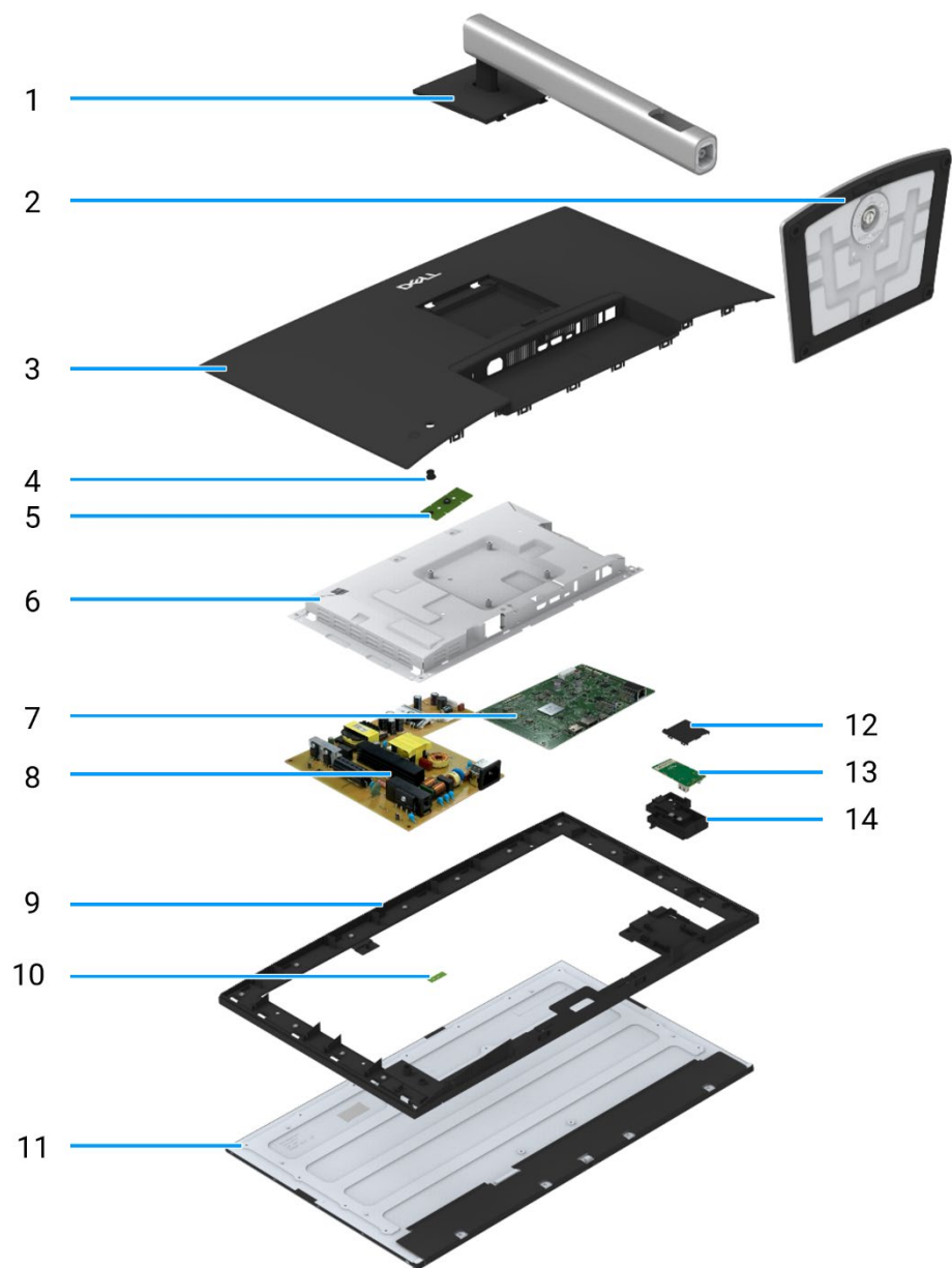
Figure 8. Major components
