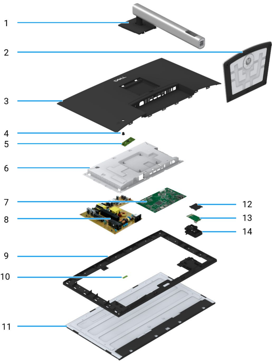
Figure 7. Major components
