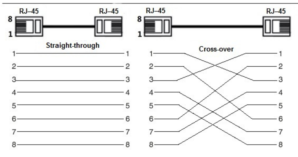
Figure 3-3 Pin description
