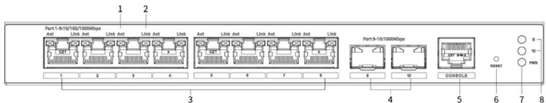
Figure 2-1 Front panel
